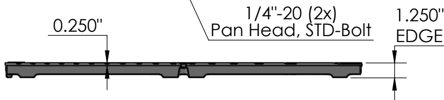
SIDE VIEW scale 1:8
