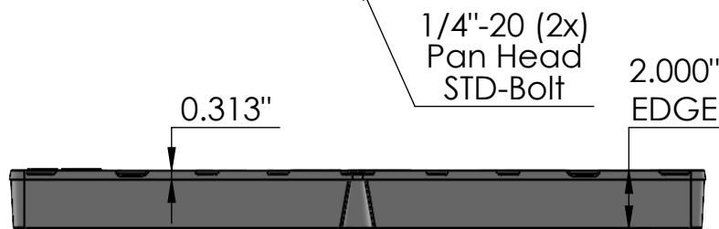
SIDE VIEW scale 1:6
